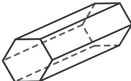
hexagonal prism
