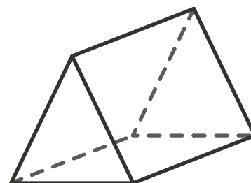
triangular prism
